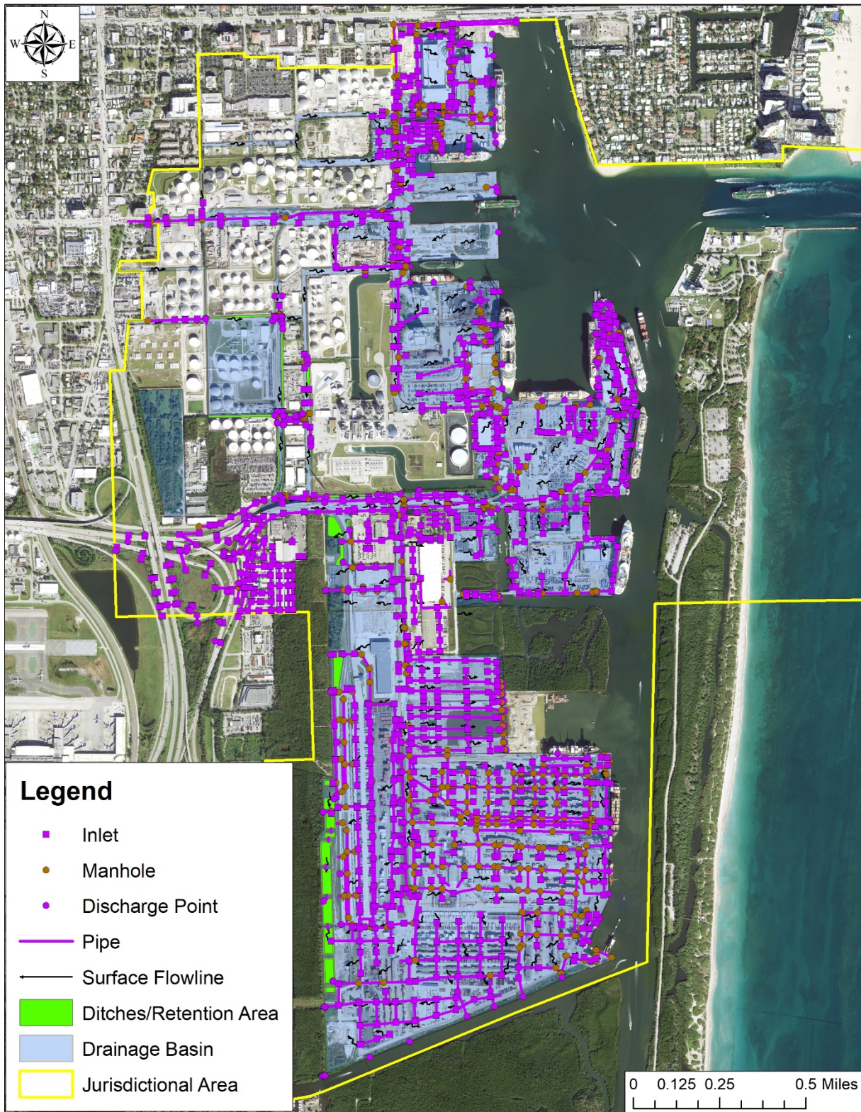
Figure P-12: Drainage Facilities (Stormwater)
