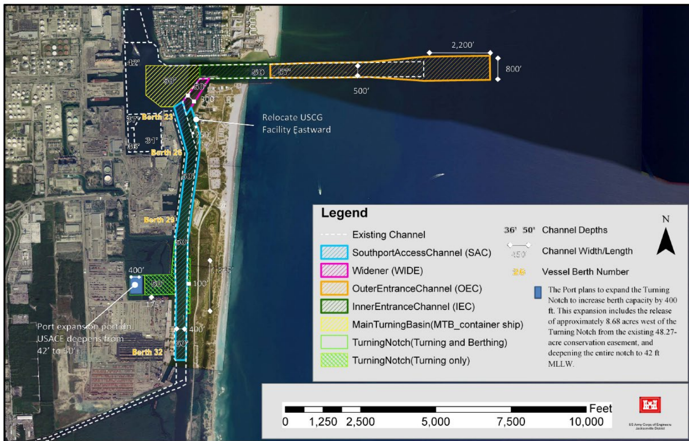
Figure P-22: ACOE Tentatively Selected Plan
