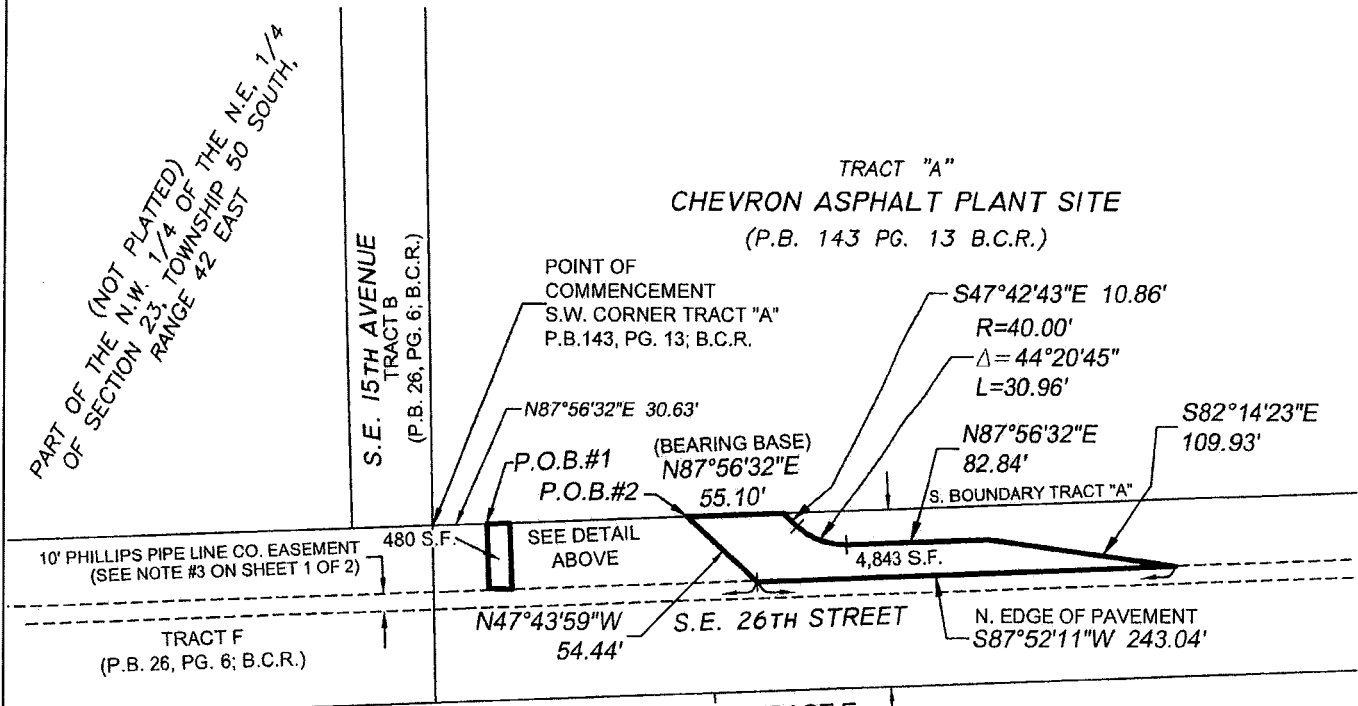
DETAIL (SCALE: 1"=40')
